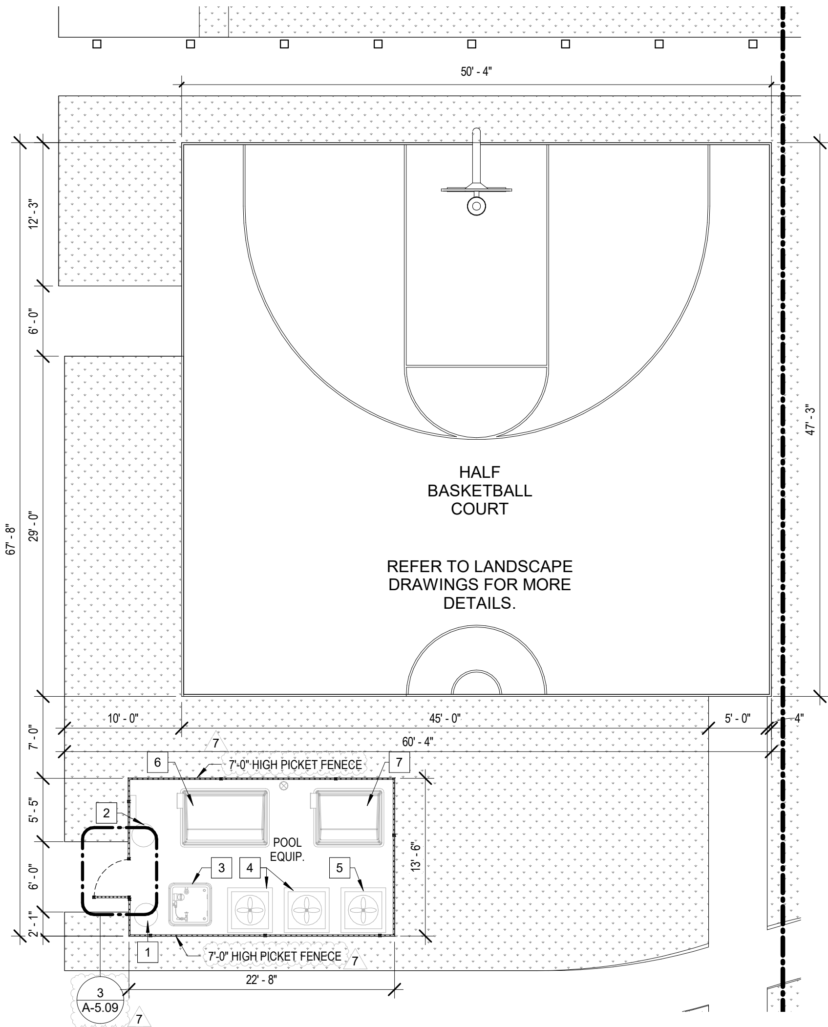
1 HALF BASKETBALL COURT- FLOOR PLAN SCALE: 1/8" = 1'-0"
