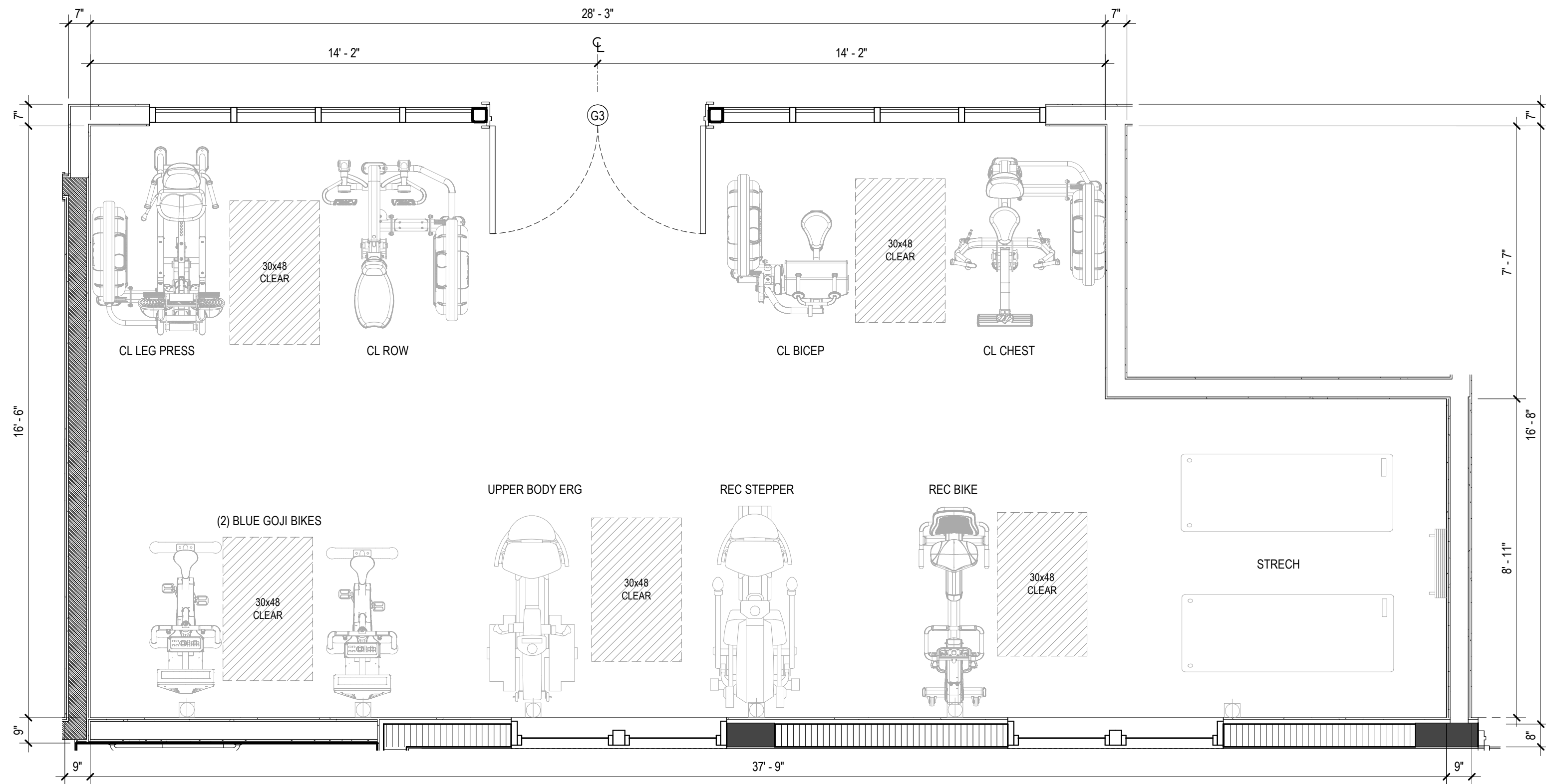
2 COMMUNITY CENTER GYM - FLOOR PLAN SCALE: 3/8" = 1'-0"
